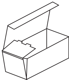
Name: FEFCO STYLE 0421 Description: Folding box with locking sides
